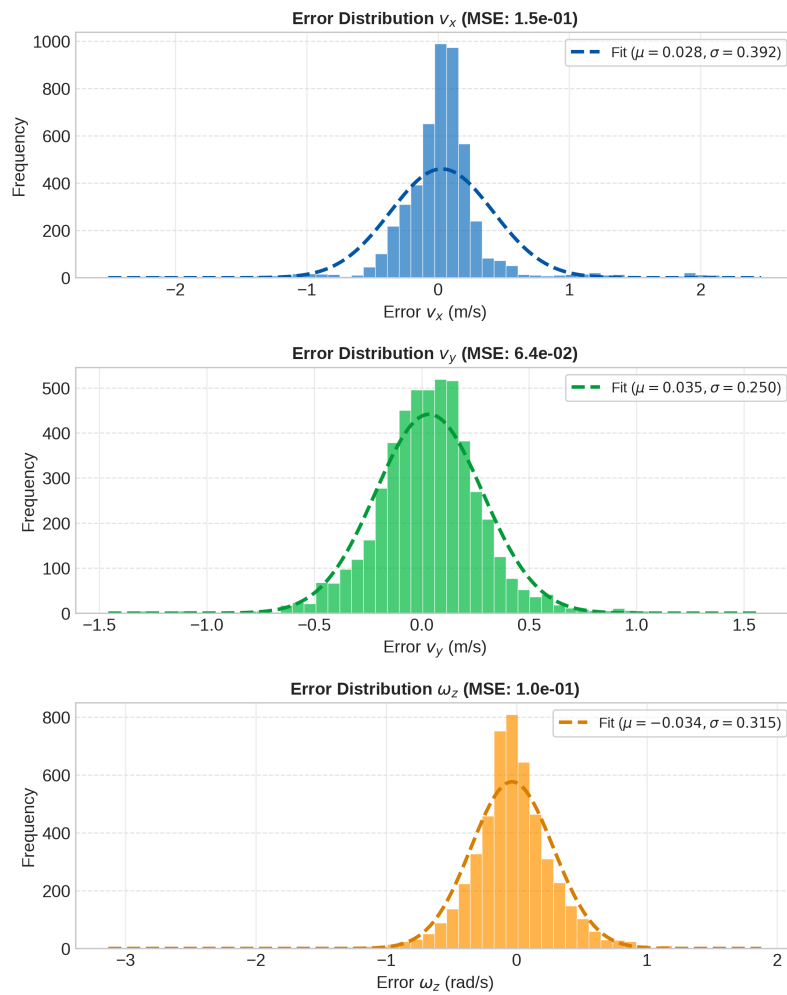
Figure 3: Linear Velocity ( v_x, v_y ) and Angular Velocity ( \omega_z ) Tracking Error Distribution
